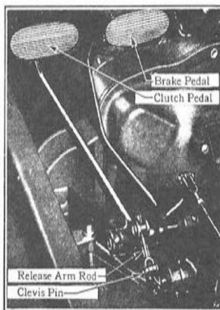
Figure 4 Clutch Pedal Adjustment
